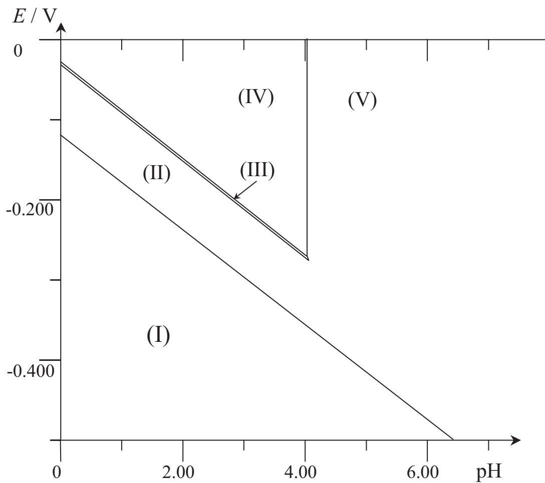
Figure 3 : Diagramme E - pH
