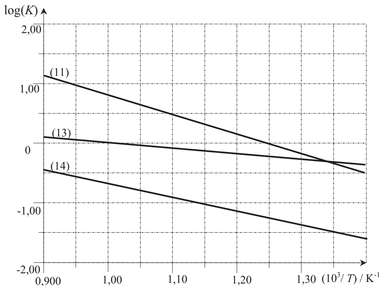
Figure 2 : \log(K) = f(1/T)
